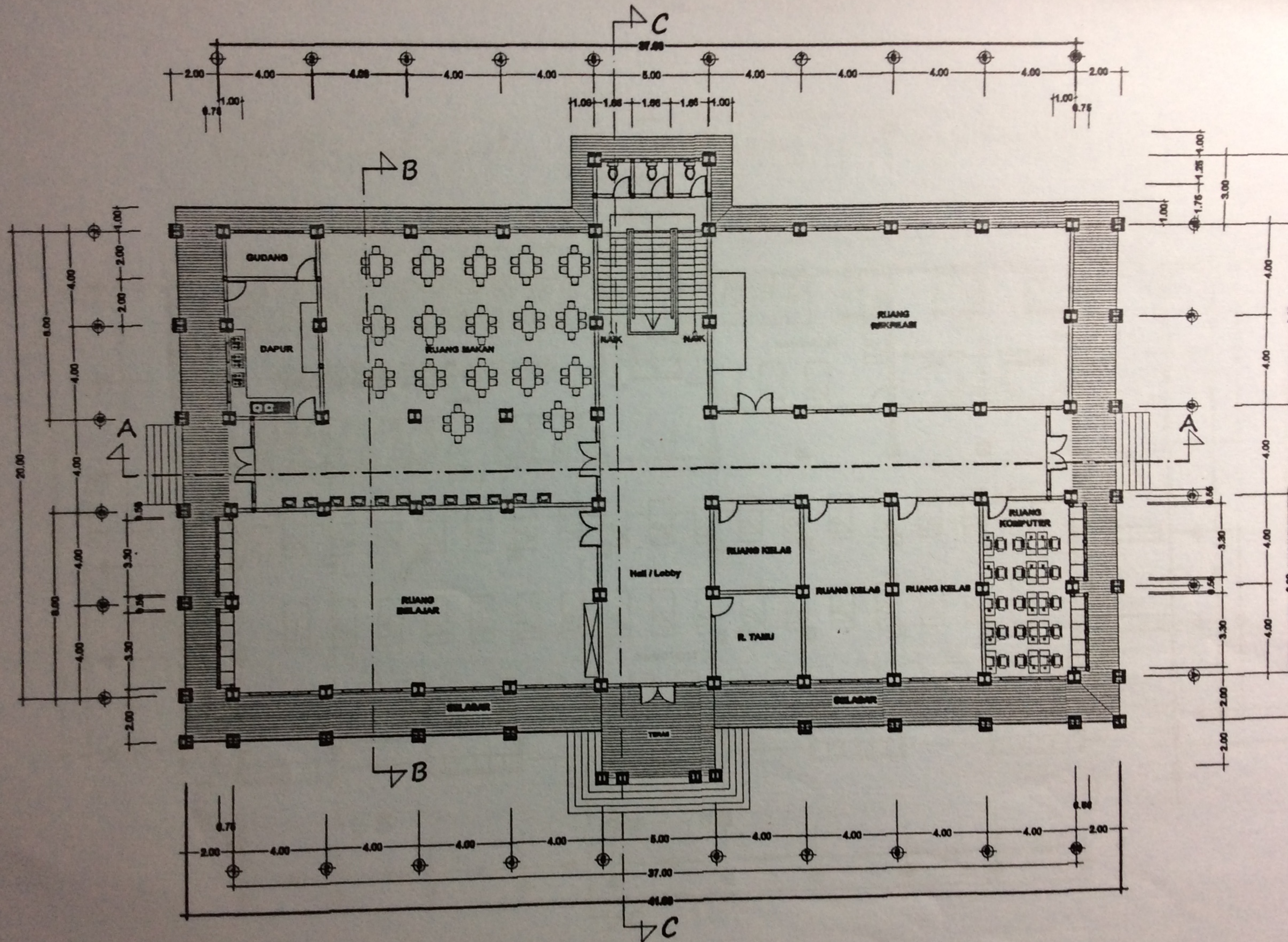
R DENAH LT. I
